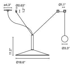
Milana 47 Counterweight
